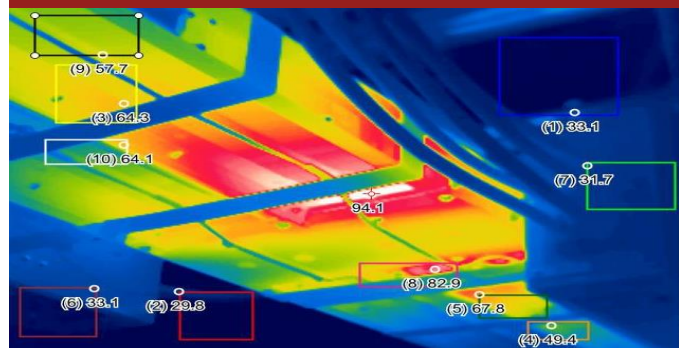
Thermal image of hot bus bar
